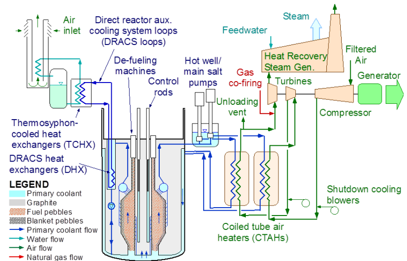
Flow schematic for Mark 1 pebble-bed fluoride high-temperature reactor
