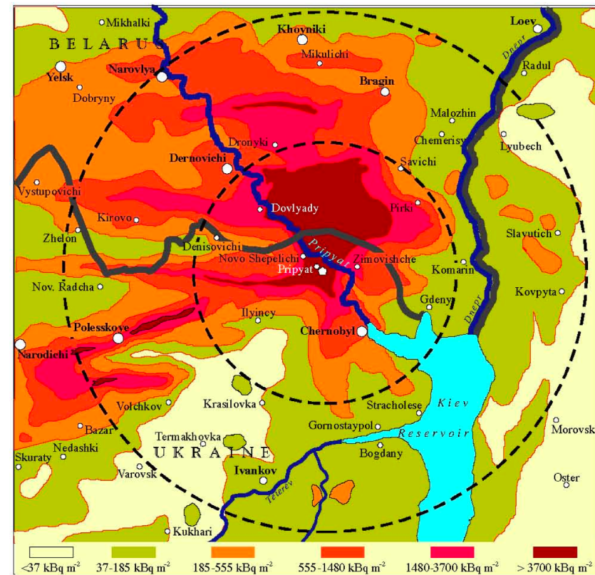
Cs-137 contamination after Chernobyl. Source: UNSCEAR, 2000
