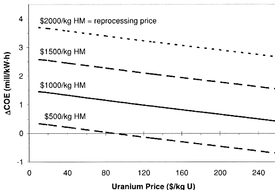
Fig. 2. The additional cost of electricity ( \Delta\text{COE} , mill/kW·h) for the reprocessing-recycle option, for reprocessing prices of $500, $1000, $1500, and $2000/kg HM, compared to the cost of electricity for the direct disposal option, as a function of the price of uranium ($/kg U).
