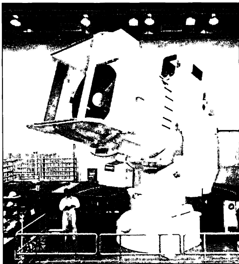
The Sealite laser beam director at the White Sands missile test range.
