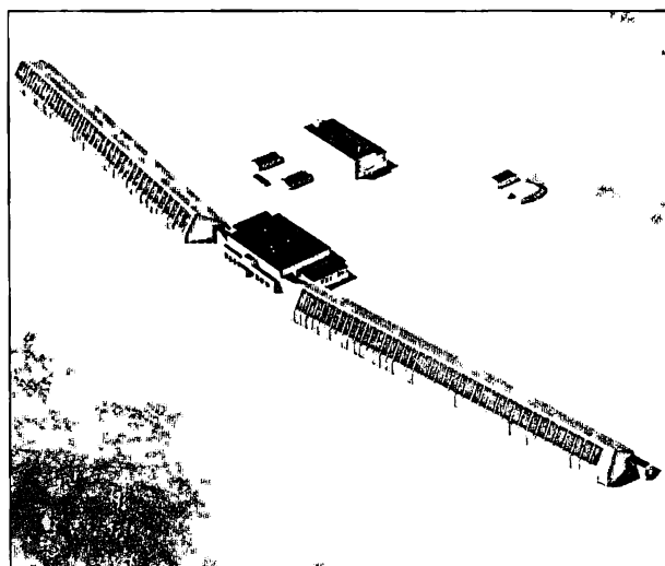
Warning Network: The Soviet Union is now replacing the aging Hen House early warning radars (right) with a network of large phased-array radars, the first of which was built near the town of Pechora (left). These radars will provide improved early warning, but their extreme vulnerability, their location, and their design features make them poorly suited for an ABM role.
